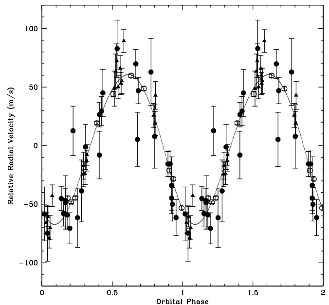
FIG. 8.—Phased radial velocities for HD 102195. The KPNO coude data are filled circles, the KPNO 2.1 m data are filled triangles, and the HET data are open circles. Two orbital cycles are shown, and each observation is plotted as two points. The best fit to the data yields an orbital period of 4.11434 days and a velocity semiamplitude of 63.4 m s ^{-1} . If the stellar mass is 0.93 M_\odot , the derived minimum planetary mass is 0.488M_J and the minimum orbital radius is 0.0491 AU. [See the electronic edition of the Journal for a color version of this figure.]
