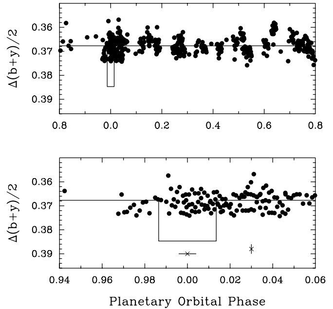
FIG. 10.— Top : Strömgren (b+y)/2 photometric observations of HD 102195 obtained during the 2005–2006 observing season with the T10 0.8 m APT at Fairborn Observatory and plotted against orbital phase of the planetary companion. The predicted time, depth, and duration of possible transits are shown schematically. The star exhibits no optical variability on the radial velocity period larger than 0.0004 mag or so. Bottom : Observations around the predicted time of transit are replotted with an expanded scale on the abscissa. The error bars are described in the text. Even very shallow transits are ruled out by these observations.
