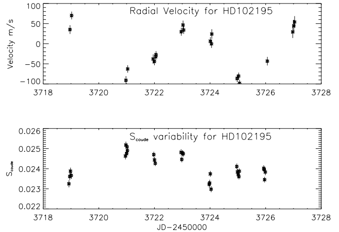
FIG. 11.—Measurements of the S_{\text{coude}} index ( bottom ) and RV ( top ) during the same observation run at Kitt Peak.
